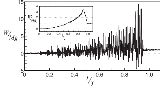
FIG. 4. The apparent weight W versus the time t . W is compared to the weight Mg of the chain, and the time t is compared to the duration T of free fall from the height L . The experiment is performed with the ball chain and the vessel is empty. Inset: filtered signal. The signal is smoothed by averaging over an interval of \pm 50 ms. [xx isn't the interval necessarily positive? xx]
