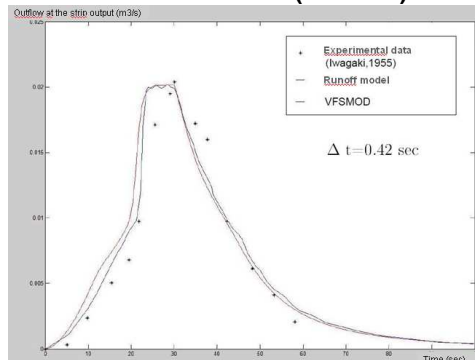
Figure 1. Iwagaki test to check the kinematic wave solving code robustness: comparison of the code with data experiments (stars) and VFSMOD simulation (blue line).
