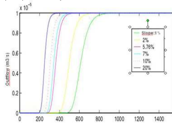
Figure 2. Sensitivity analysis of the output flow (m 3 /s) to the slope, from 1% to 20%.
