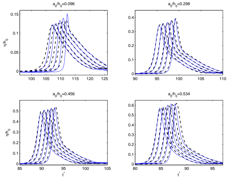
Figure 8: Nonlinear shoaling of solitary waves propagating over a beach - Time series of the free surface elevation for the solitary wave propagating over the 1:30 sloping beach. (—) experimental data, (- - -) numerical results, with t^* = t(g/h_0)^{1/2} .
