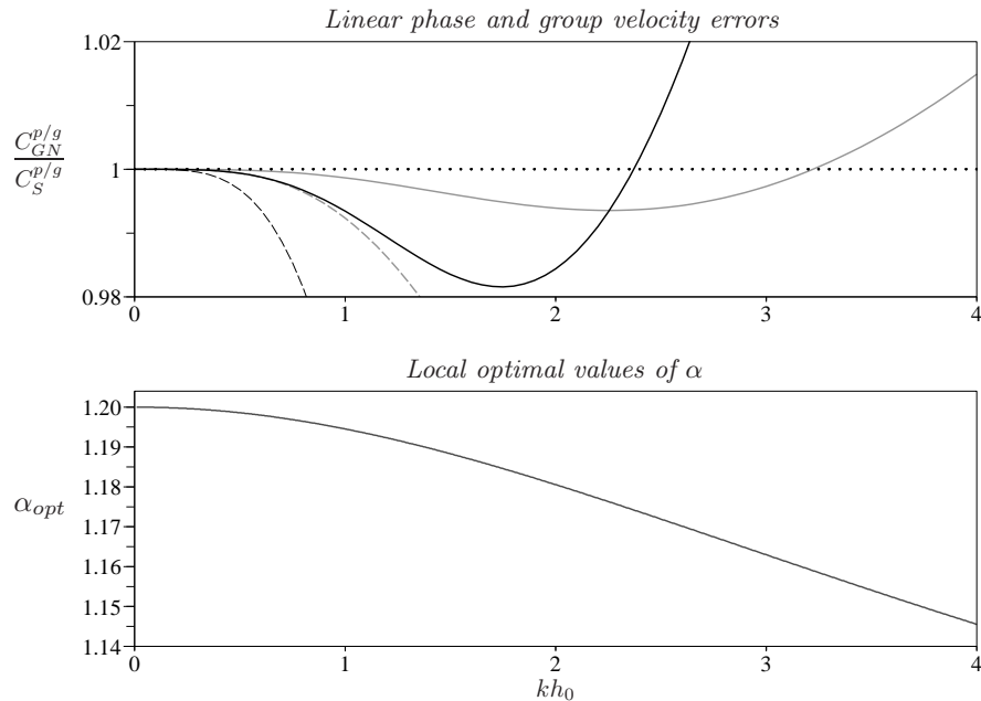
Figure 2: Top: linear phase velocity (black) and group velocity (grey) errors for \alpha = 1.159 (full line, global optimal value) and \alpha = 1 (dashed line, original model). Bottom: local optimal values of \alpha for kh in [0; 4] .
