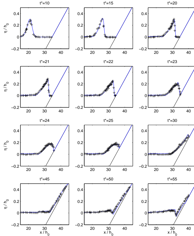
Figure 9: Comparisons of model predictions (—) and experimental snapshots (+) for a breaking solitary wave with non-dimensional initial incident amplitude a_0/h_0 = 0.28 , on a 1 : 19.85 constant slope beach investigated by Synolakis (1987), with t^* = t(g/h_0)^{1/2} .
