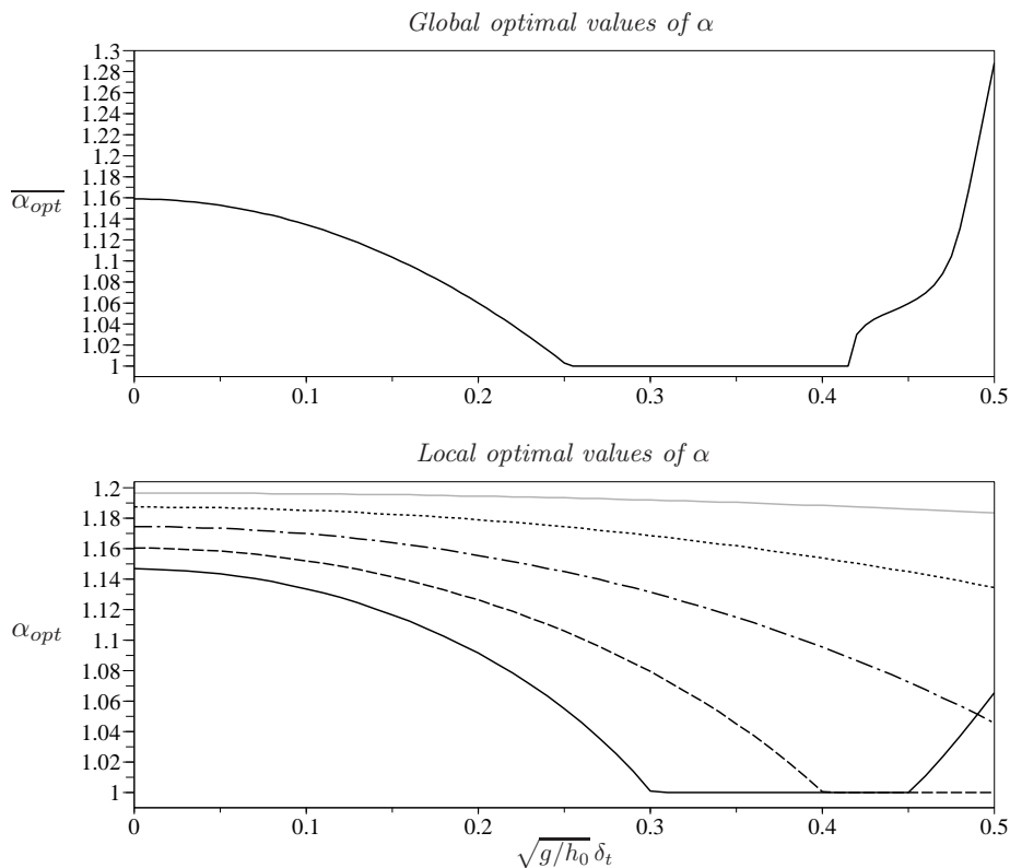
Figure 3: Top: global optimal values of \alpha against \tilde{\delta}_t . Bottom: local optimal values of \alpha against \tilde{\delta}_t for kh_0 = \pi/4 (full grey line), kh_0 = \pi/2 (dotted line), kh_0 = 3\pi/4 (dash-dotted line), kh_0 = \pi (dashed line), kh_0 = 5\pi/4 (full black line).
