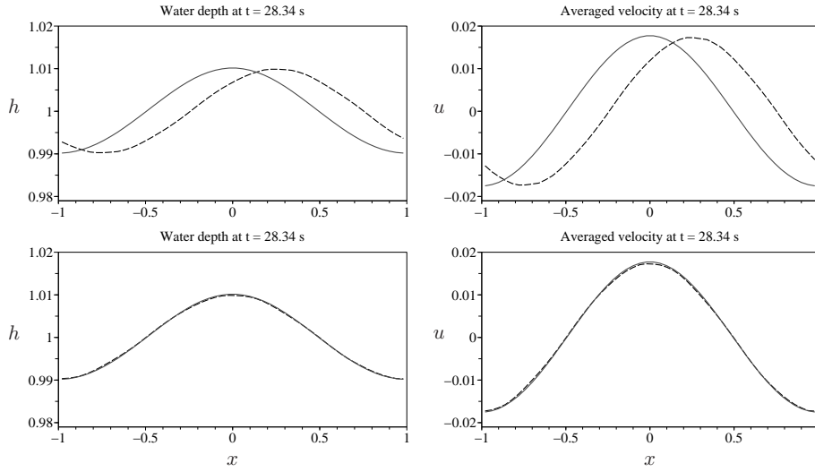
Figure 5: Numerical results at t = 25T , model with \alpha = 1.16 (top) and \alpha = 1.153 (bottom) in dashed line, reference solution in full line.
