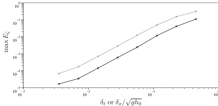
Figure 4: Propagation of a solitary wave over a flat bottom, maximum of the relative error on the free surface elevation. Case a/h_0 = 0.05 in black, case a/h_0 = 0.2 in grey.
