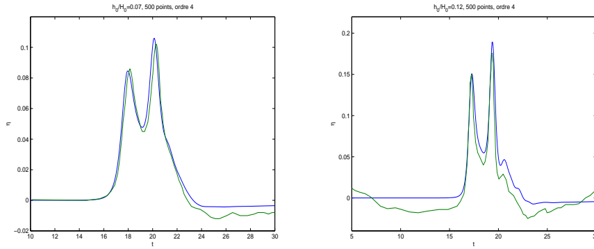
Figure 7: Reflection of a solitary wave against a vertical wall. Time series of the free surface at x = 17.75 m for a = 0.07 (left) and a = 0.12 (right): comparison between numerical results (blue line) and experimental data (green line).
