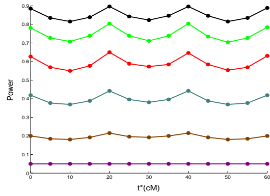
Figure 3: Power as a function of t^* and the number nz of non zero. From top to bottom, nz = 5, 4, 3, 2, 1, 0 ( I = 5 , \lambda = 2 , \sigma = 1 , npaths = 100000 ).
