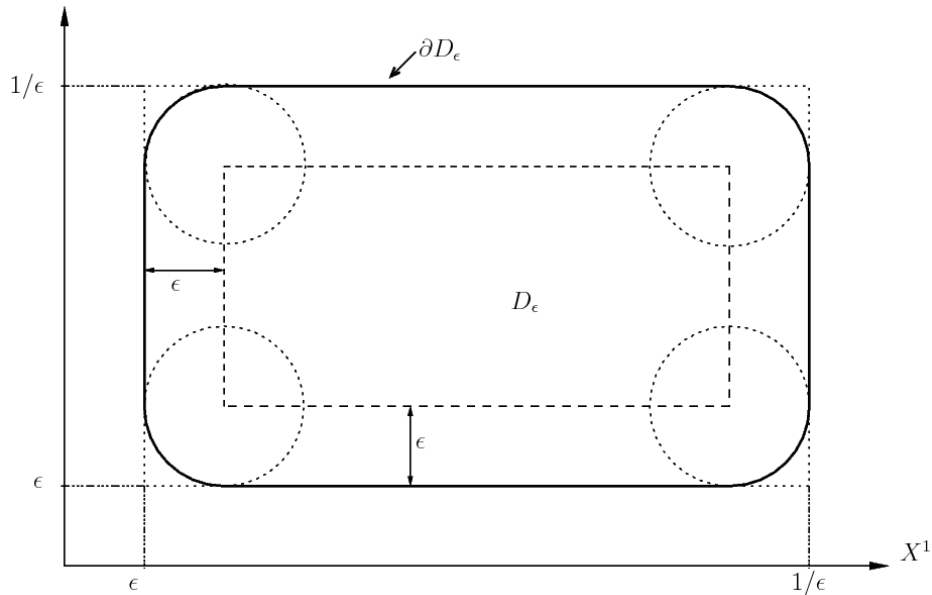
Figure 5: Definition of D_\epsilon
