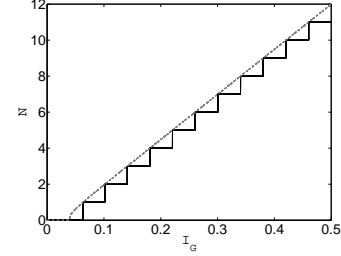
Fig. 4. The rate code generated by the ganglion cells: the rate code N = f(I_G) (solid line) and the real spiking frequency F = f(I_G) (dotted line). Simulations are made for the following parameter values: \delta = 4 , g_G = 10^{-2} , and c_G = 10^{-2} .
