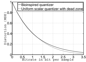
Fig. 6. Rate/distortion trade-off: Comparison between the uniform scalar quantizer with dead zone (dotted line) and the bioinspired quantizer with gain control.
