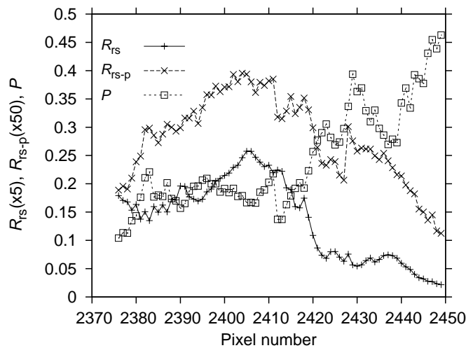
Fig. 4. Evolution of R_{rs} , R_{rs-p} , and P along a transect in the Rio de la Plata estuary (represented by the red line in Fig. 2a).
