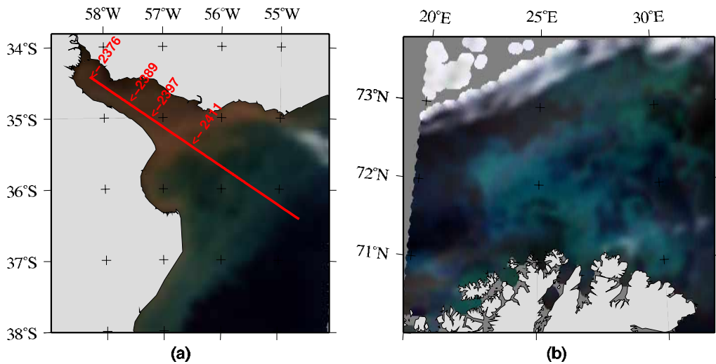
Fig. 2. POLDER2 selected scenes of RGB composites, over (a) the Rio de la Plata estuary (26 of May 2003), and (b) off Norway in the Barents sea (19 of July 2003). The red line in panel a corresponds to a transect specifically examined, and the numbers represent the pixel number (see text for details).
