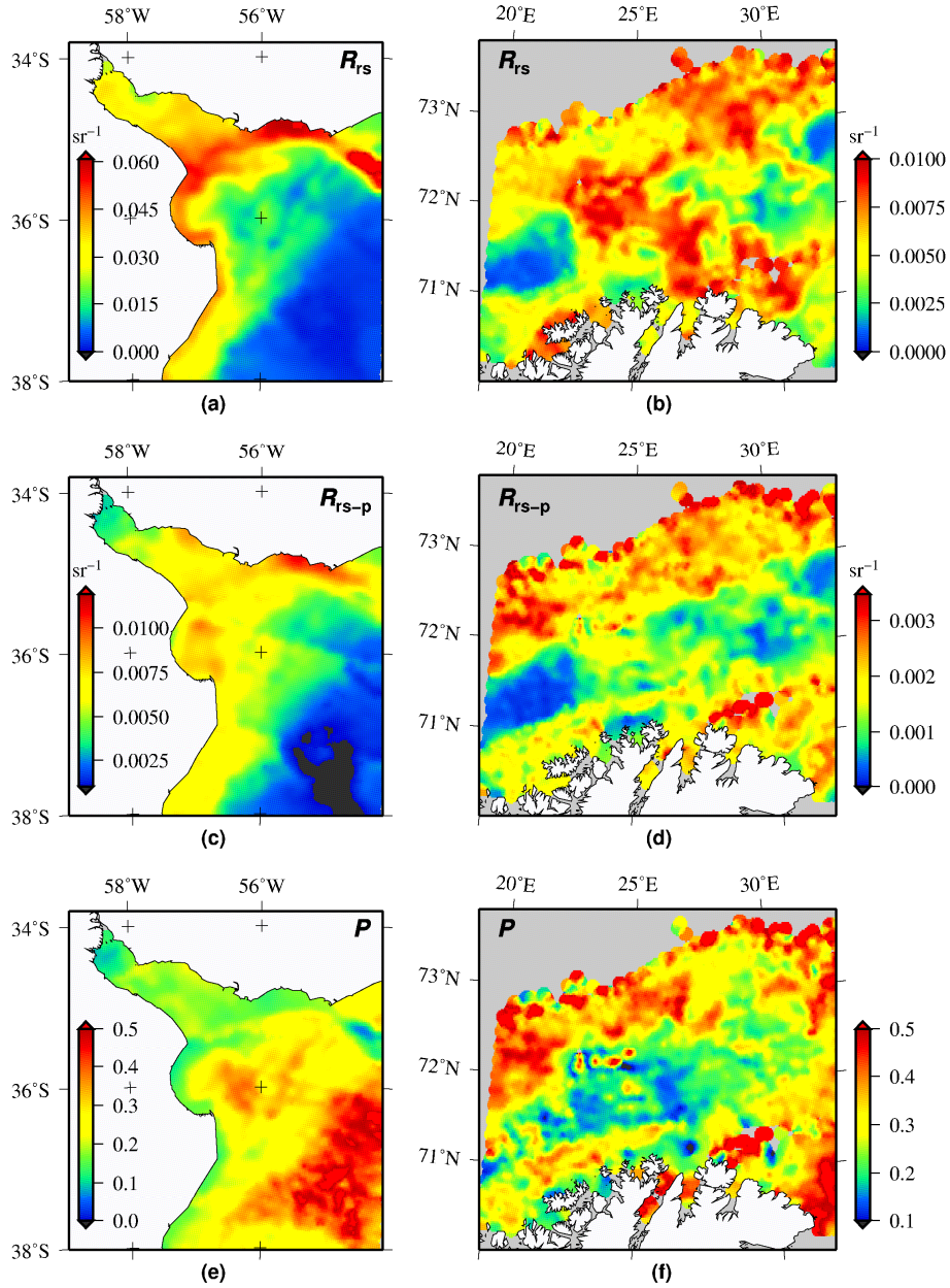
Fig. 3. Maps of R_{rs} , R_{rs-p} , and P at 670 nm for the Rio de la Plata estuary (left column), and the Barents Sea areas (right column).
