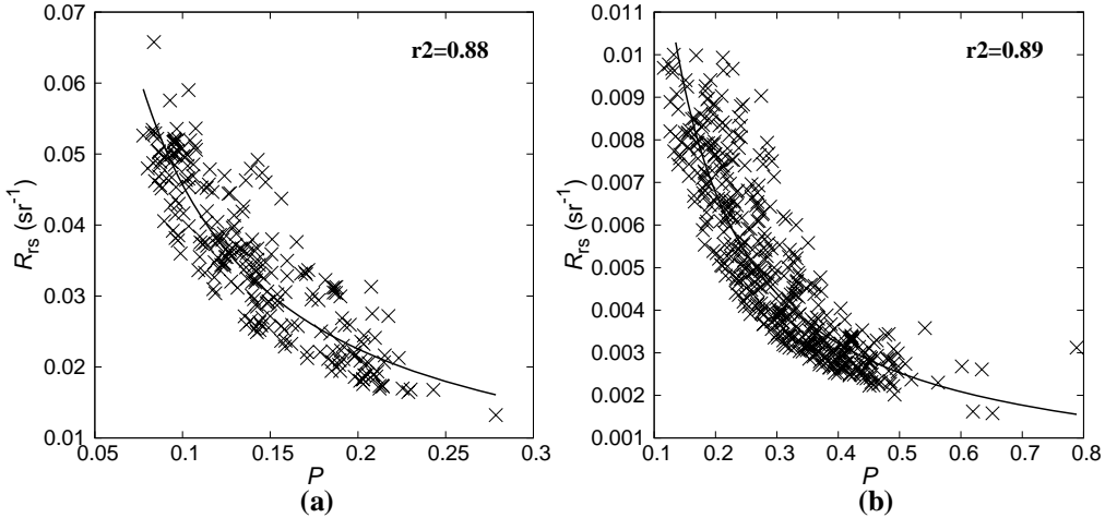
Fig. 5 Scatter plot of R_{rs} as a function of P at 670 nm for (a) the Rio de la Plata estuary, and (b) the Barents Sea areas. The black lines in panel a and b correspond to the fits described by the equations 2 and 3, respectively. The square correlation coefficient ( r^2 ) is given. Note the different scales of the two panels.
