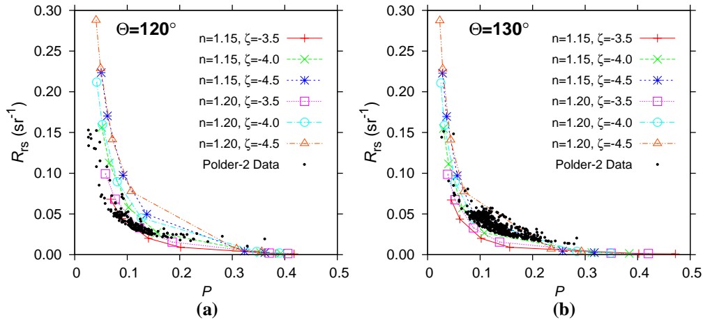
Fig. 6. Variation of R_{rs} as a function of P for the value of the scattering angle of (a) 120^\circ and (b) 130^\circ for the Rio de la Plata estuary waters. The colored symbols represent data obtained from the radiative transfer simulations performed for different values of the refractive index, n , and PSD slope, \zeta , as indicated. The black dots represent the data obtained from POLDER-2 observations. Note that the P values are lower than those presented in Fig. 1 for which the calculations did not account to multiple scattering.
