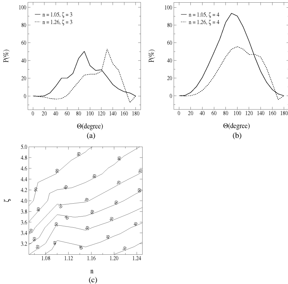
Fig. 1. Degree of polarization P (in %) as a function of the scattering angle, \theta , for two extreme refractive index relative to waters, n , and for two different values of the PSD slope, \zeta : a) \zeta=3 , and b) \zeta=4 . c) Contour diagrams of P(90) as a function of the parameters n (x-axis), and \zeta (y-axis). Note that the P values presented in this figure are not affected by multiple scattering in contrast to what happens in the ocean.
