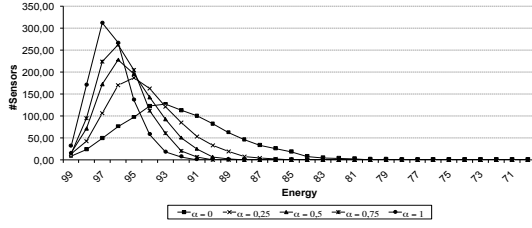
Figure 6: Energy Distribution after the first duty-cycle ( n=1000 ).
