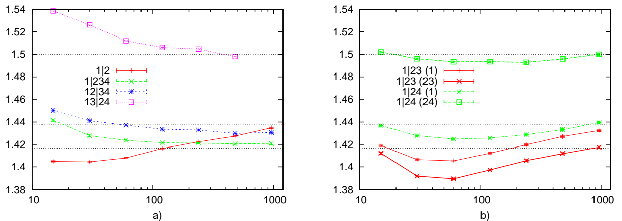
Figure 1: Effective exponents obtained for different interfaces. The three dashed lines correspond to 1 + 10/24, 1 + 7/16, 3/2 as discussed in text.
