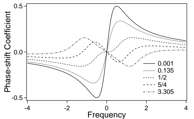
Figure 3: Same as Fig.2 for the phase-shift coefficient \varphi(\Omega) in \alpha/2 units.
