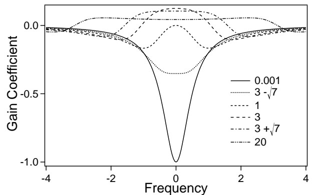
Figure 2: Gain coefficient g(\Omega) in \alpha/2 units as a function of \Omega in 1/T_1 units for T_2 = 2T_1 . The different curves are labeled by the corresponding value of the normalized intensity I_{cw} .
