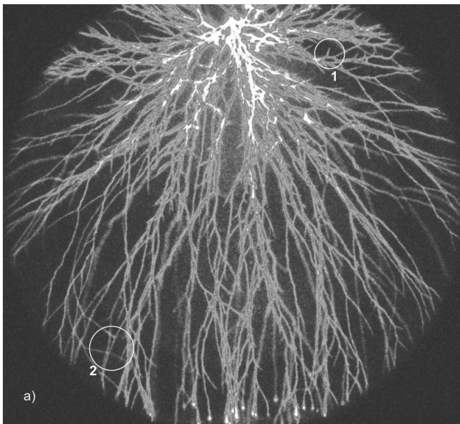
FIGURE 1a). ICCD image of a point-to-plane corona discharge in a 16 cm gap at 400 mbar in nitrogen with about 0.2 % oxygen 14 . The streamers are thinner than in air, form very short branches, e.g., .in circle 1, and possibly reconnect, see circle 2.
