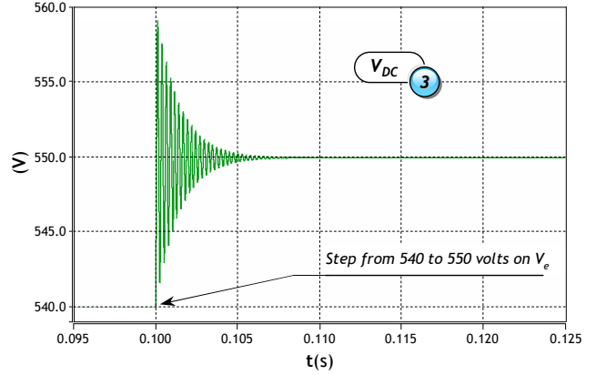
(a) Simulation with the parameters defined in point 3 ( K_p = 10 and R = 5\Omega )
