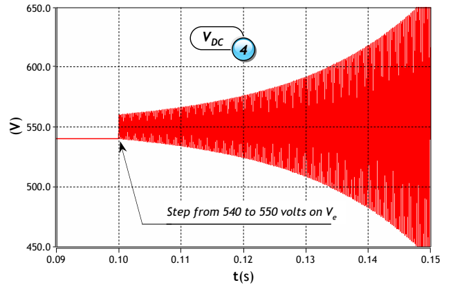
(b) Simulation with the parameters defined in point 4 ( K_p = 10 and R = 20\Omega )
