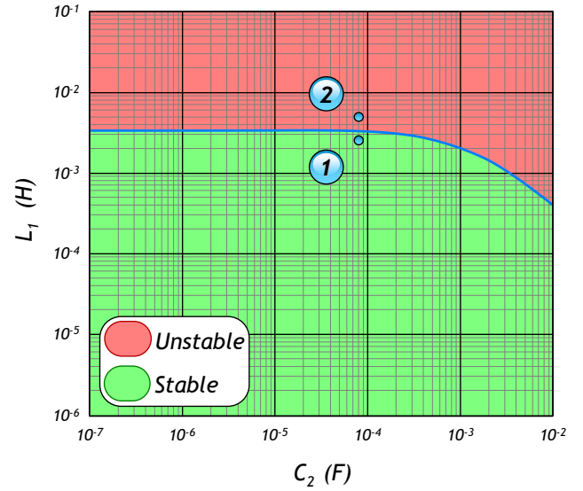
Fig. 12. Stability analysis with a sweep on \{L_1, C_2\} parameters
