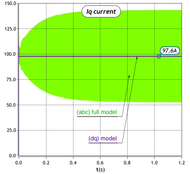
Fig. 6. Current regulation on q axis
