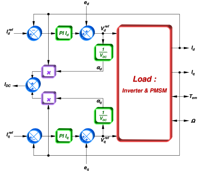
Fig. 4. Control part
