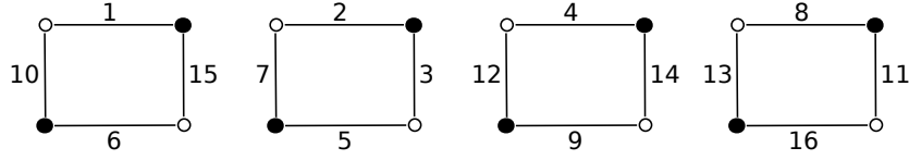
FIGURE 3. Polygons associated to the couple (S_1, S_2) .
