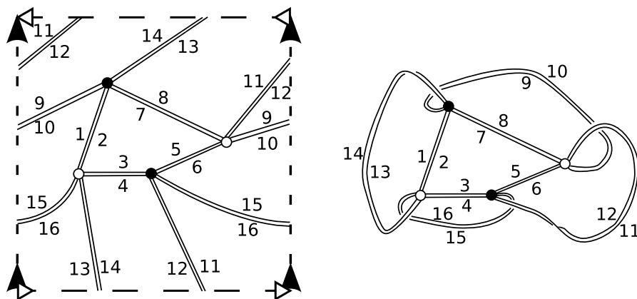
FIGURE 4. Example of a labeled map on Klein bottle.
