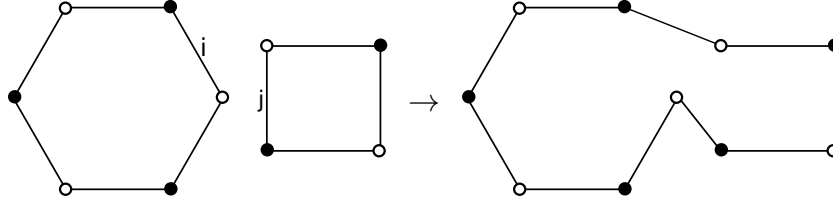
FIGURE 1. \mathcal{L}(S_0, S_1) and \mathcal{L}(S'_0, S_1) in the first case of proof of Lemma 3.8.
