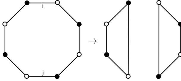
FIGURE 2. \mathcal{L}(S_0, S_1) and \mathcal{L}(S'_0, S_1) in the first case of proof of Lemma 3.8.
