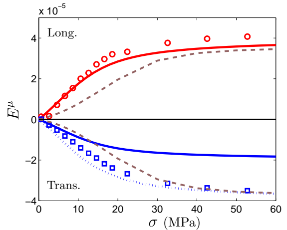
Fig. 13. \Delta E effect for an iron-cobalt alloy: longitudinal and transverse magnetostriction strain as a function of the applied stress \sigma , modeling (line) and experimental (points) results. Plain line for isotropic strain and dot line (transverse direction) for configuration energy effect. Dashed lines: Results obtained with a full multiscale model with configuration energy effect [5, 15, 16].
