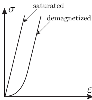
Fig. 1. Illustration of \Delta E effect on a tensile stress-strain curve ( \varepsilon is the total strain).
