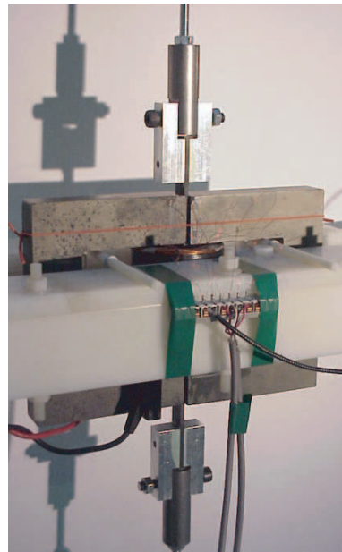
Fig. 7. Apparatus for measurement of magnetostriction under applied stress - with articulated heads.
