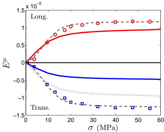
Fig. 12. \Delta E effect for an iron-silicon steel: longitudinal and transverse magnetostriction strain as a function of the applied stress \sigma , modeling (line) and experimental (points) results. Plain line for isotropic strain and dot line (transverse direction) for configuration energy effect. Dashed lines: Results obtained with a full multiscale model with configuration energy effect [5, 15, 16].
