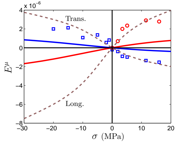
Fig. 11. \Delta E effect for Ni-Zn ferrite: longitudinal and transverse magnetostriction strain as a function of the applied stress \sigma , modeling (line) and experimental results. Dashed lines: Results obtained with a full multiscale model [12].
