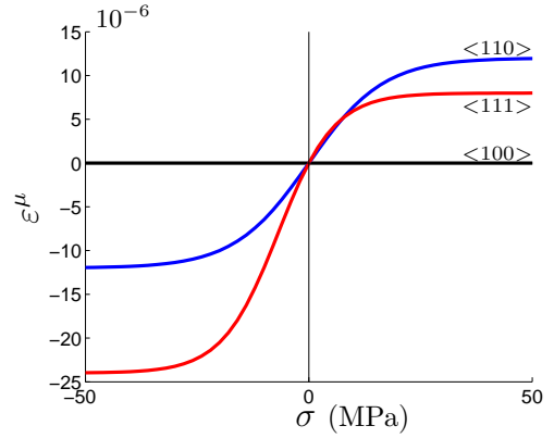
Fig. 5. \Delta E effect in the case of nickel single crystal.
