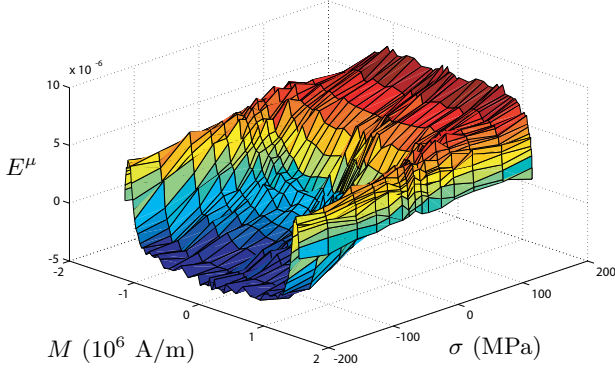
Fig. 8. Influence of uniaxial stress on the anhyseretic longitudinal magnetostrictive behavior of pure iron [11].
