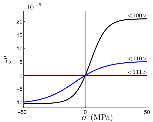
Fig. 3. \Delta E effect in the case of iron single crystal.
