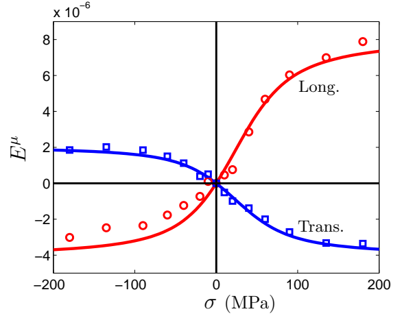
Fig. 10. \Delta E effect for pure iron: longitudinal and transverse magnetostriction strain as a function of the applied stress \sigma , modeling (line) and experimental results.
