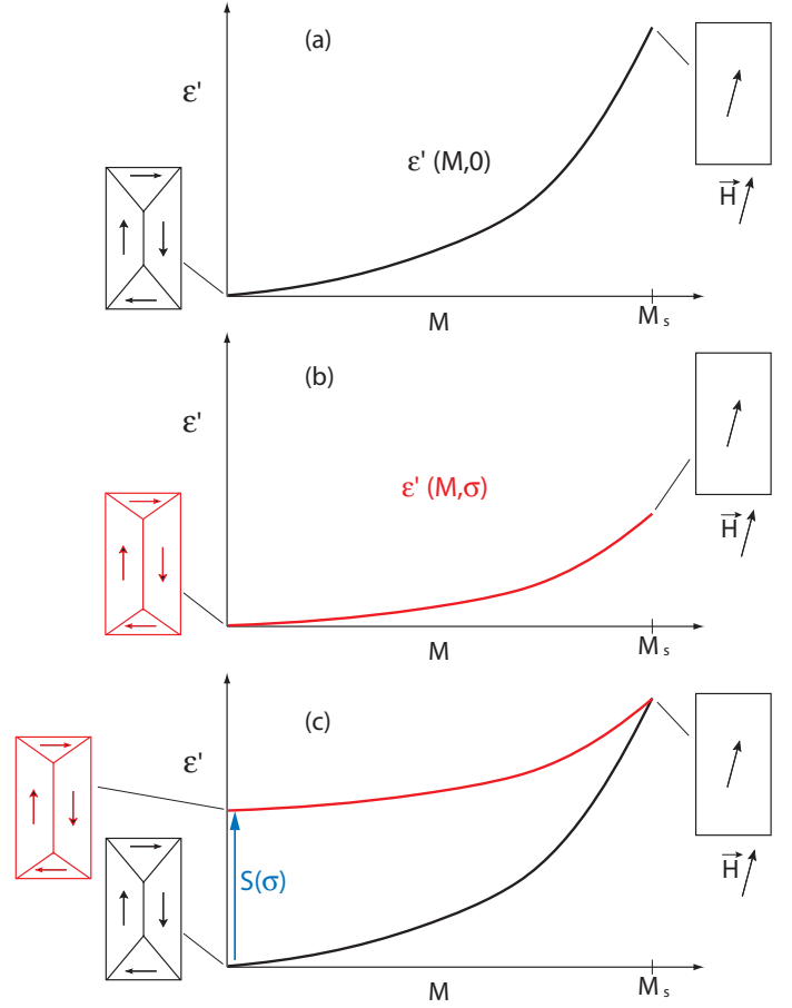
Fig. 6. Schematic view of the measured deformation \varepsilon' and associated domain structure; (a) zero stress; (b) with \sigma applied stress; (c) shift of the \sigma applied stress curve to get the same saturation value.
