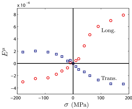
Fig. 9. \Delta E effect for pure iron - longitudinal and transverse behaviors.
