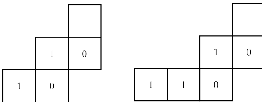
FIGURE 2. The staircases \dots 1010\dots and \dots 11010\dots
