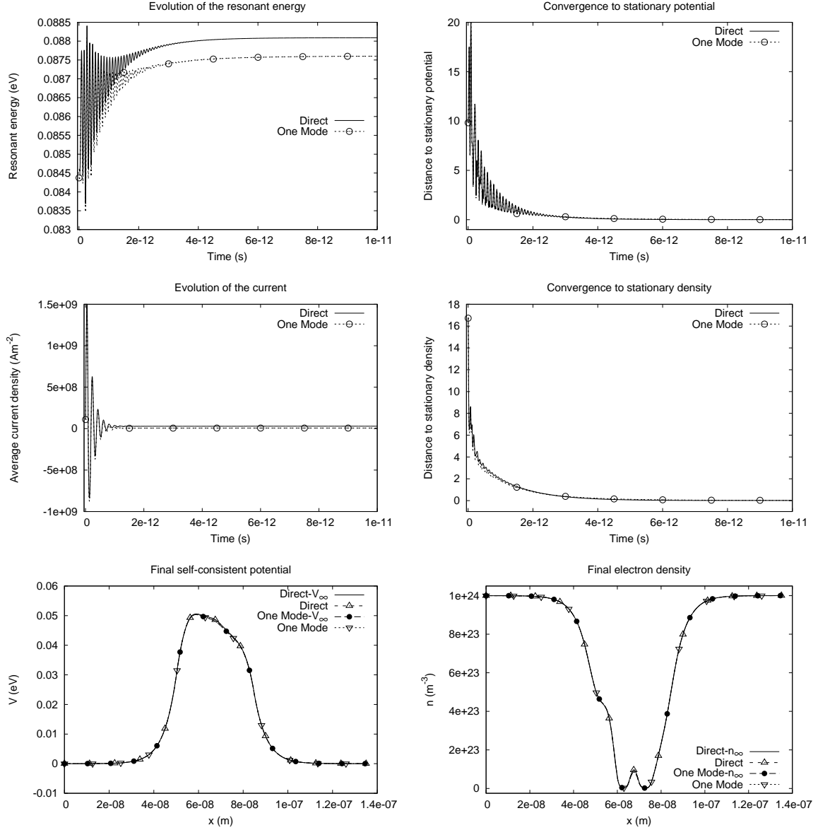
Figure 7: For M = 500 , P = 3900 , P' = 300 , \Delta t = 2 \times 10^{-15} s , t_{tot} = 5 \times 10^3 and, for the methods considered, are depicted from left to right: Evolution of the resonant energy, Evolution of the potential relative distance (5.1) to the stationary solution, Evolution of the average current density defined by (5.3), Evolution of the density relative distance (5.2) to the stationary solution, Self-consistent potential at final iteration t_{tot} , and Electron density at final iteration t_{tot} .
