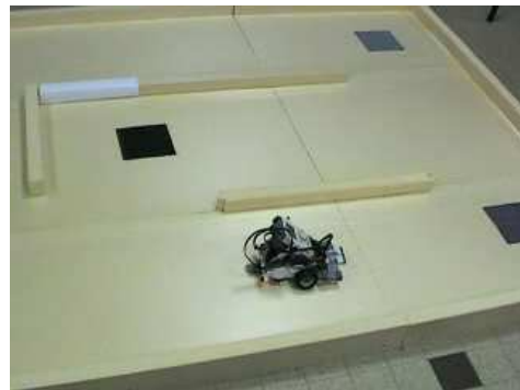
Figure 2. LEGO®MINDSTORMS®NXT robotics project.
