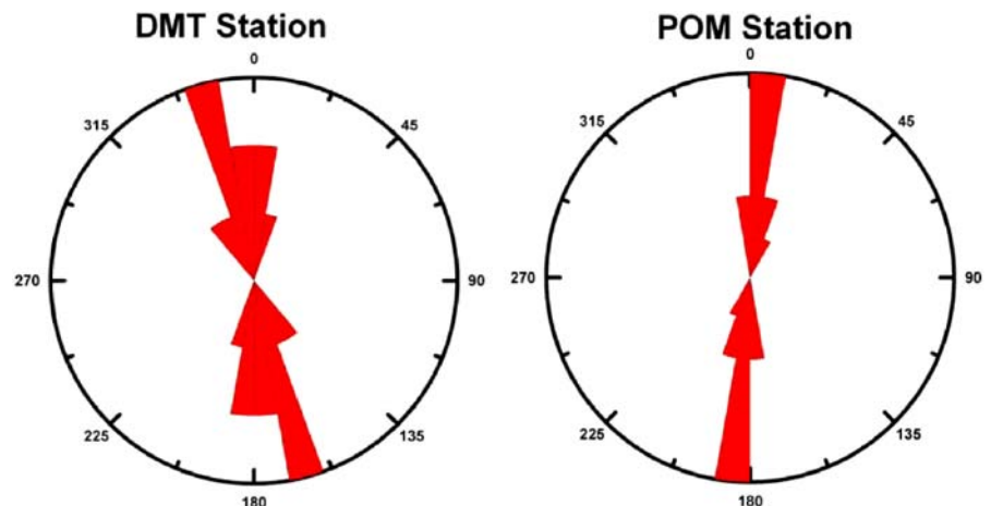
Fig. 6 Rose diagrams at Mt. Etna for the 1988 dataset at stations DMT and POM
