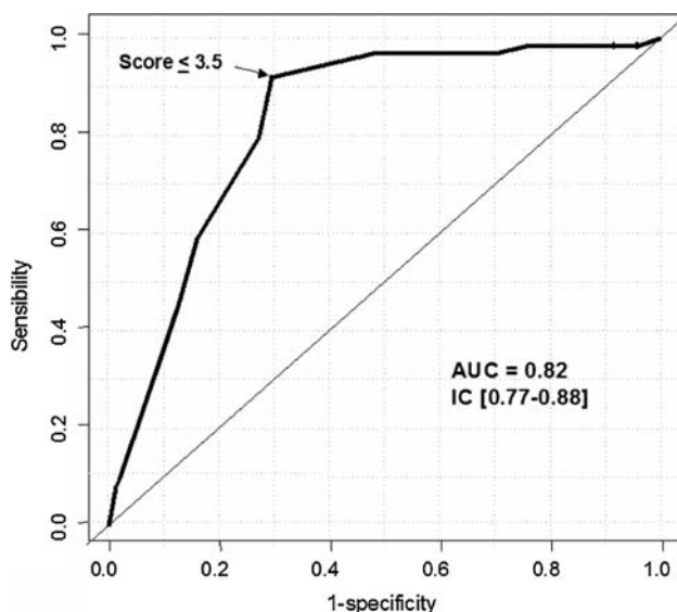
Fig. 1 A receiver operating characteristics (ROC) curve assessing the discriminatory capacity in the Tenon score
