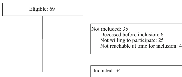
Fig. 1 Study flow-chart
