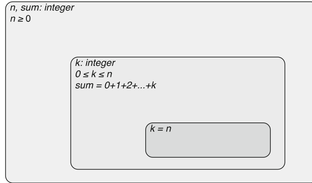
Fig. 5. Nested situations
