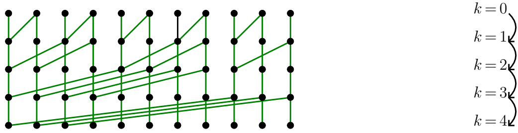
Figure 3. Schematic representation of the conversion Newton to monomial for d = 11
