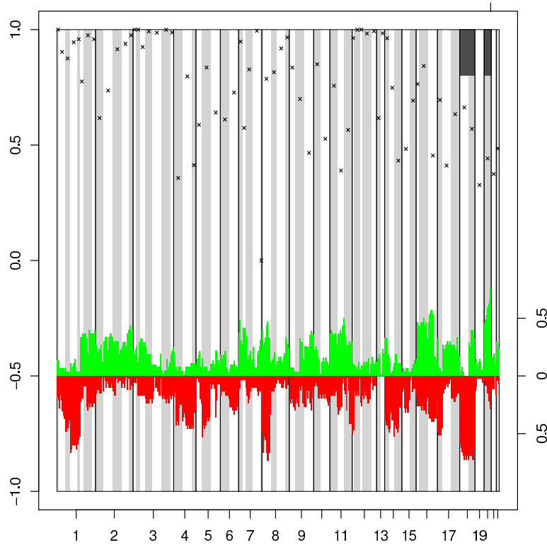
Figure 5: Clustering plus testing plot for Data2. See caption Figure 4.
