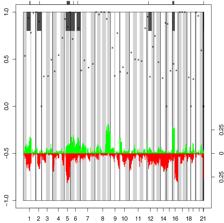
Figure 4: Clustering plus testing plot for Data1. Chromosomes are indicated on the bottom axis and are separated by solid lines. Alternating light-grey and white bars demarcate different clusters. Crosses show the association coefficient \tilde{\gamma} for each cluster (scale on left axis). Dark-grey bars indicate significant clusters, tick marks at the top axis mark significant regions within such clusters. Significance level for clusters and regions is \alpha = 0.1 . At the bottom the absolute difference between the proportion of gains in the two groups (green) and the absolute difference between the proportion of losses (red) is plotted (scale on right axis).
