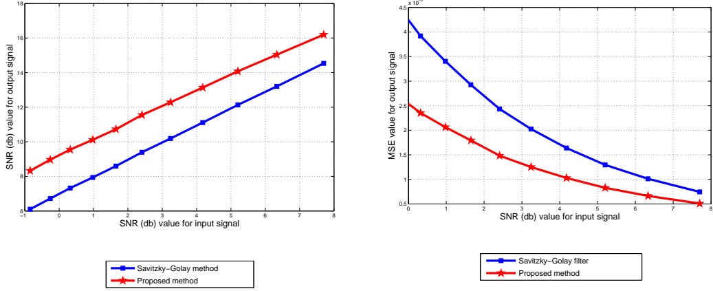
(a) SNR values in Savitzky-Golay method in comparison (b) MSE values in Savitzky-Golay method in comparison to proposed method using finite difference scheme to proposed method
