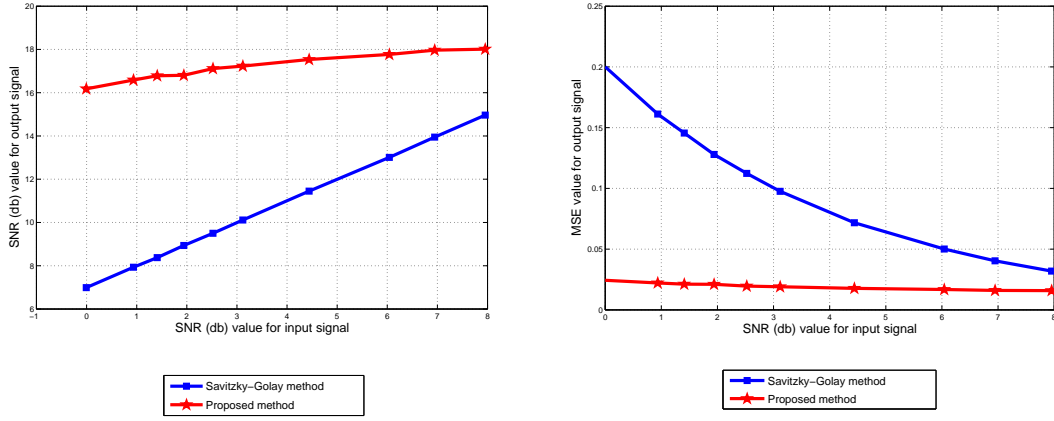
(a) SNR values in Savitzky-Golay method in comparison (b) MSE values in Savitzky-Golay method in comparison to proposed method
