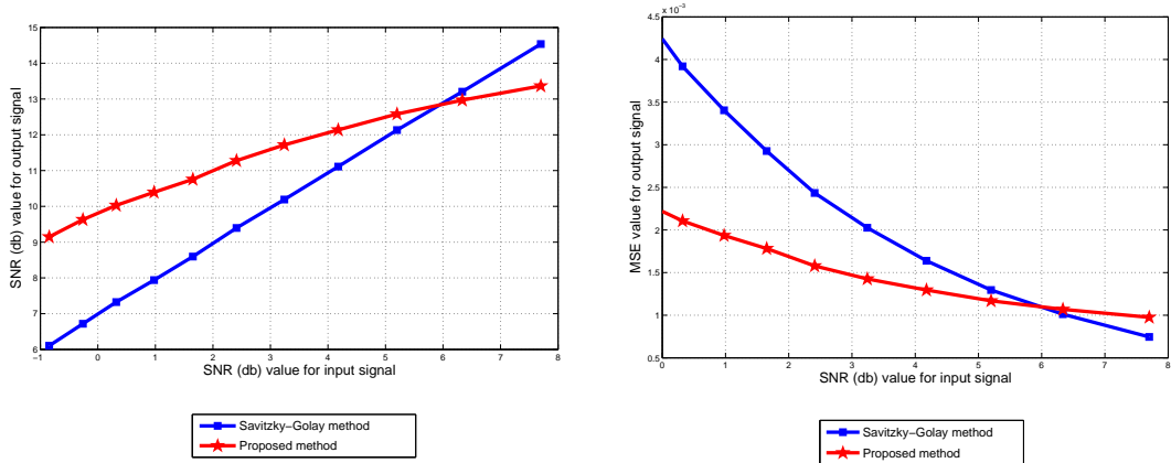
(a) SNR values in Savitzky-Golay method in comparison (b) MSE values in Savitzky-Golay method in comparison to proposed method
