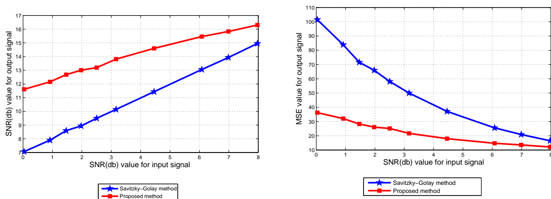
(a) SNR values in Savitzky-Golay method in comparison to (b) MSE values in Savitzky-Golay method in comparison to proposed method
