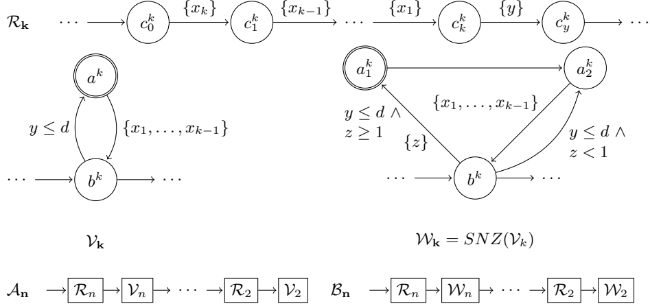
Fig. 1. Gadgets for \mathcal{A}_n and \mathcal{B}_n = SNZ(\mathcal{A}_n) .
