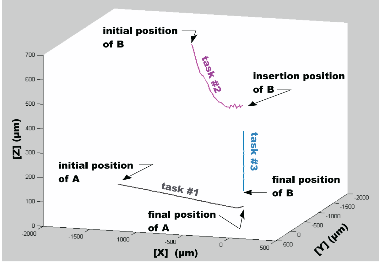
Figure 14: Illustration of the different trajectories obtained with the pose-based visual control.
