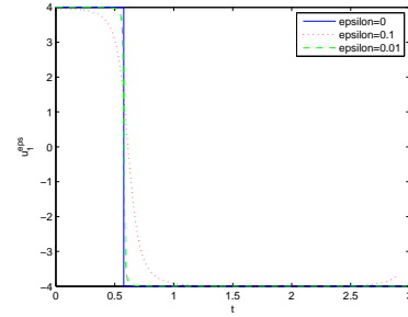
Figure 8: Control
