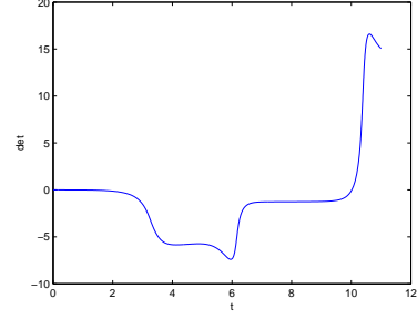
Figure 18: Determinant ( \varepsilon = 0.1 )
