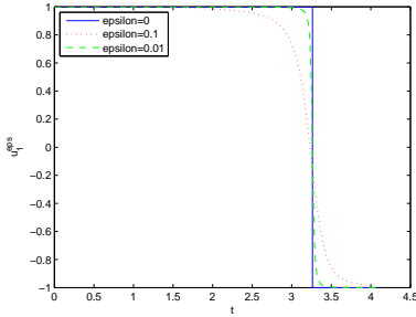
Figure 17: Control
