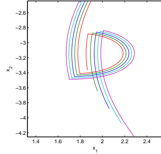
Figure 14: Zoom on the overlap of the flow at the third switching time
