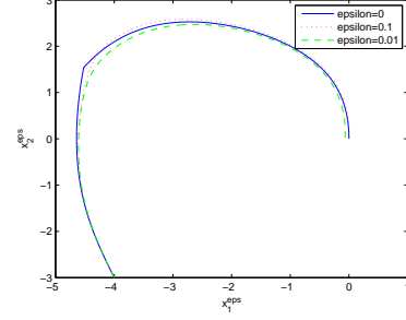
Figure 6: Trajectory
