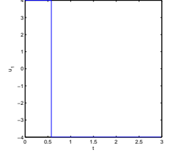
Figure 3: Optimal control
