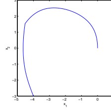
Figure 2: Optimal trajectory
