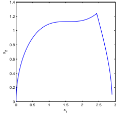
Figure 11: Optimal trajectory
