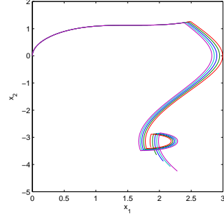
Figure 13: Extremal field, t \in [0, 11]
