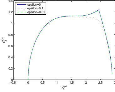
Figure 15: Trajectory
