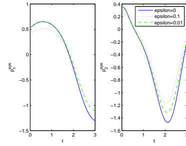
Figure 7: Adjoint vector
