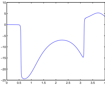
Figure 9: Determinant ( \varepsilon = 0.01 )
