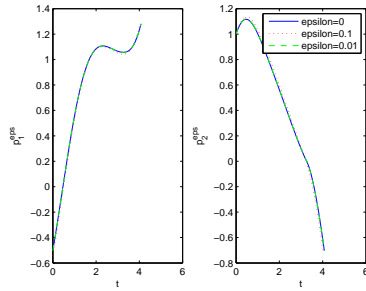
Figure 16: Adjoint vector
