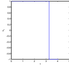
Figure 12: Optimal control
