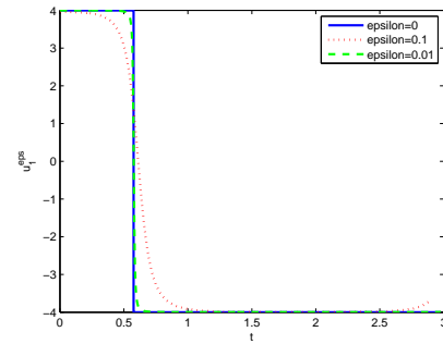
Figure 9: Control
