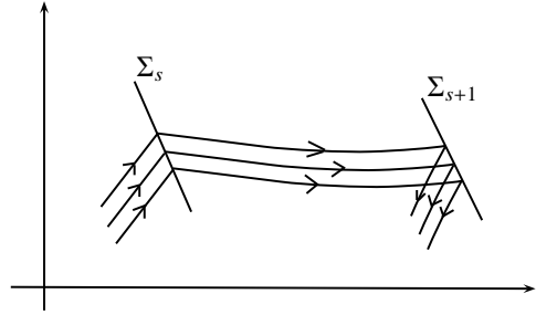
Figure 1: Field of extremals
