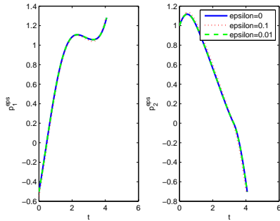
Figure 17: Adjoint vector
