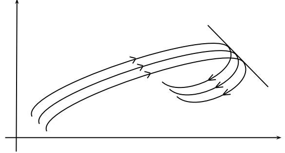
Figure 2: Field of extremals in the smooth case
