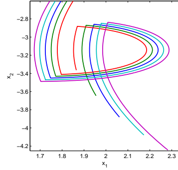
Figure 15: Zoom on the overlap of the flow at the third switching time
