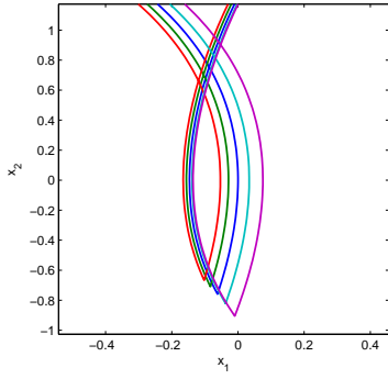
Figure 6: Overlap of the flow
