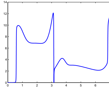
Figure 11: First singular value of J^\varepsilon(t) ( \varepsilon = 0.01 )
