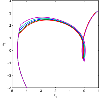
Figure 5: Extremal field t \in [0, 4]
