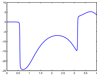
Figure 10: Determinant ( \varepsilon = 0.01 )
