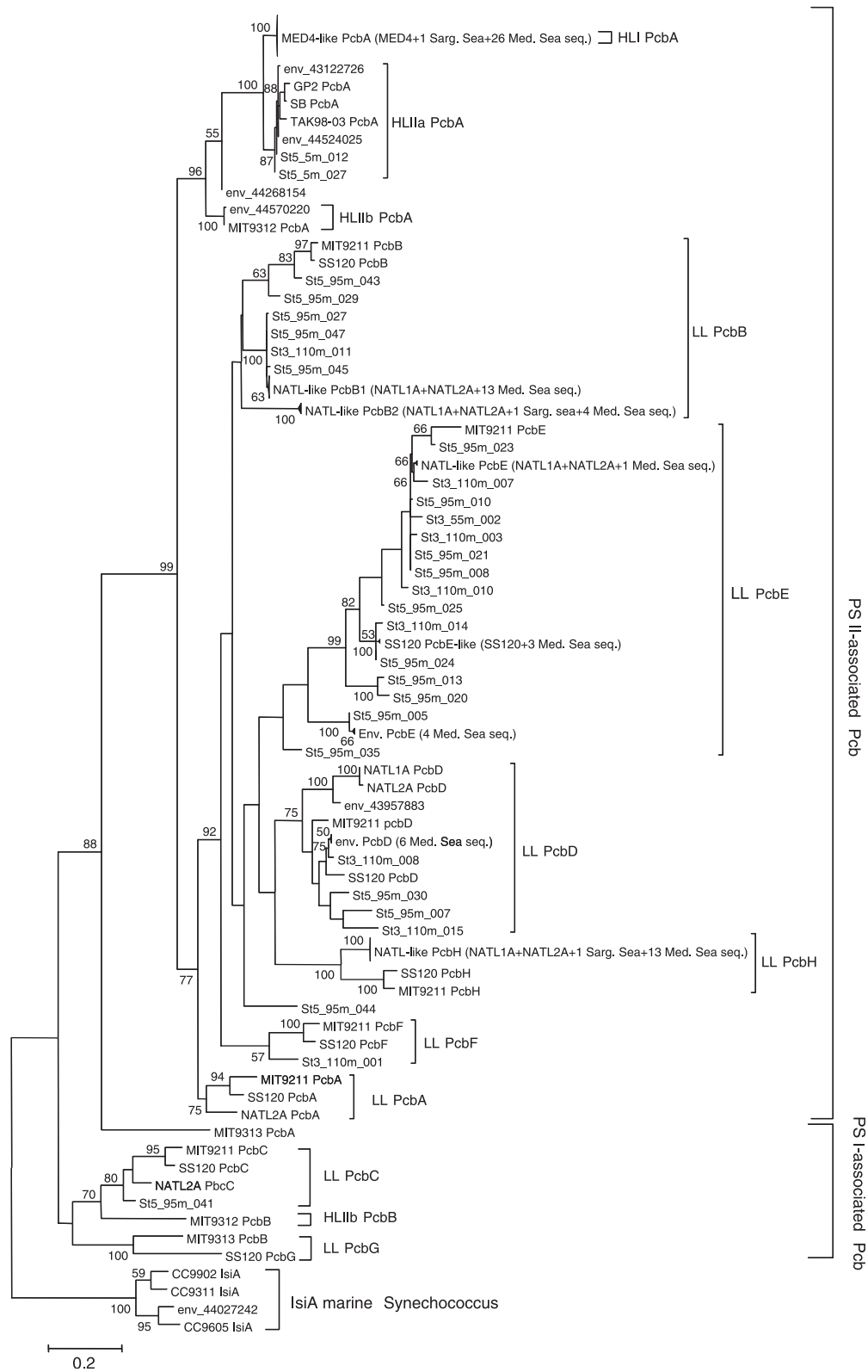
Fig. 5. Maximum likelihood tree of Pcb amino acid sequences (all gaps were excluded from the alignment) obtained with the PHYLML software. Only bootstrap values > 50% for 1000 replicates are shown. Details on sequences used in this analysis are listed in Tables 1 and 2. For readability, clusters containing a large number of closely related sequences are shown as vertical lines or triangles (depending on the variability among sequences) and the content of these clusters is indicated between parentheses. Med., Mediterranean; Sarg., Sargasso; seq., sequences.
