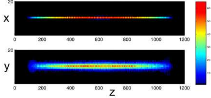
FIG. 2: (Color online) Simulated CCD-image of 70 ions laser cooled along the x -axis and trapped in the pseudo-potential associated to the rf field defined in IIB, with an anisotropy characterized by \alpha = 10^{-3} . The pixel size is 1 \mu\text{m} and the signal associated to one pixel is proportional to the number of scattered photons in this pixel, integrated over 10 ms. The picture is projected on the (x, z) plane (top) and on the (y, z) plane (bottom).
