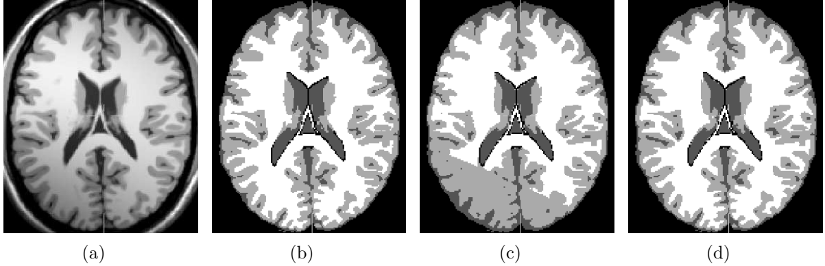
Figure 6: Segmentation results of the Brainweb T1-weighted image only corrupted by intensity inhomogeneity. (a) Original image, (b) Brainweb segmentation ground truth, (c) FCM segmentation, (d) NL-FCM segmentation ( m_j = 8 and n_j = 8 ).
