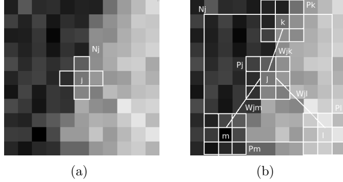
Figure 4: Comparison of (a) the R-FCM [Pha01] and (b) the NL approaches. In this example, the area around the voxel j is much more similar to the one of voxel k than the ones of voxels m and l . Therefore, the weight w_{jk} will be higher than the weights w_{jm} and w_{jl} .
