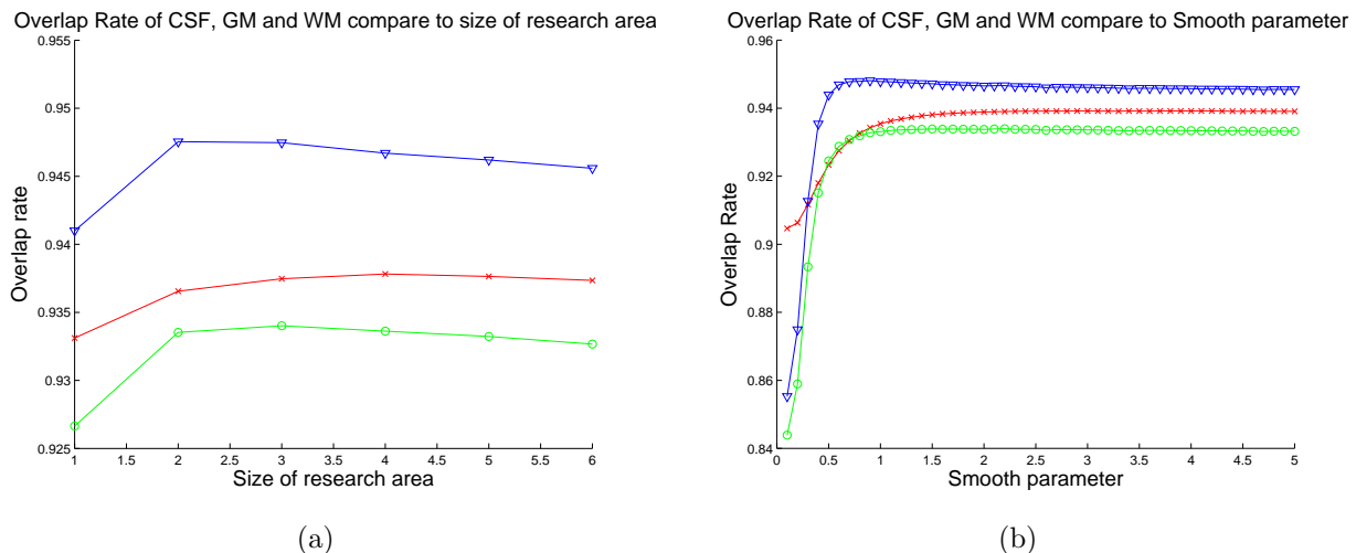
Figure 7: Influence of NL regularisation parameters. Application on the Brainweb T1-weighted image with 9% Rician noise. (a) Overlap rate w.r.t. the value of n_j^r and (b) overlap rate w.r.t. the smoothing parameter \alpha . Legend: GM ( \circ ), WM ( \nabla ), CSF ( \times ).
