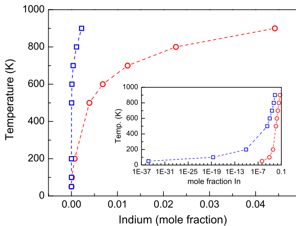
Fig. 10. Prewetting (squares) and binodal (circles) lines in the Al–In monotectic system. The two curves get closer when the temperature decreases, but they do not cross. This is highlighted in the insert where x -axis is in logarithmic scale.
