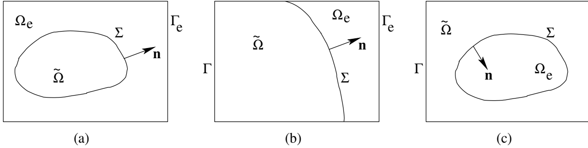
Figure 1. Configurations for embedding the original domain \tilde{\Omega} inside the fictitious domain \Omega = \tilde{\Omega} \cup \Sigma \cup \Omega_e .
