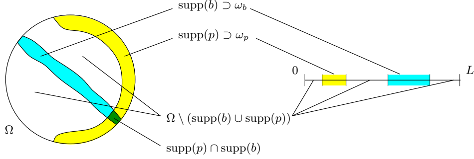
Figure 2: Some one and two dimensional geometric situations covered by Theorem 1.2 (i) Locally, the equations satisfied by u_1 and u_2 are
