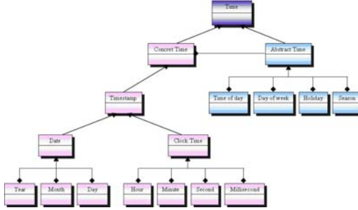
Fig. 2. A simple schema of the time model
