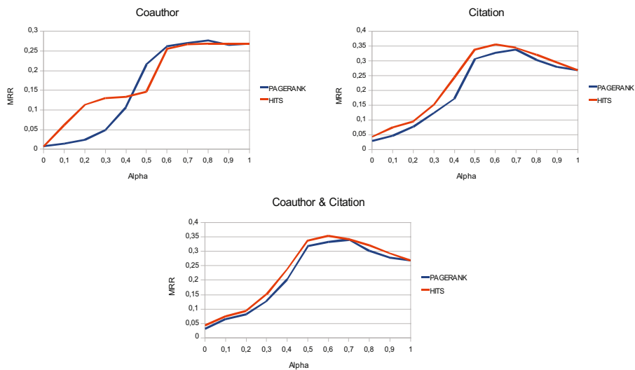
Fig. 3. Parameter tuning using most cited relevance assumption
