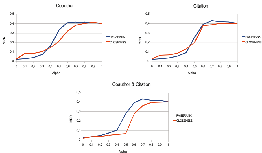
Fig. 4. Parameter tuning using most downloaded relevance assumption
