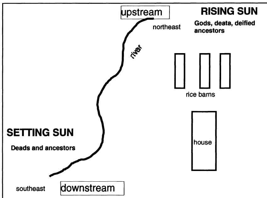
Figure 1. Toraja coordinates.
