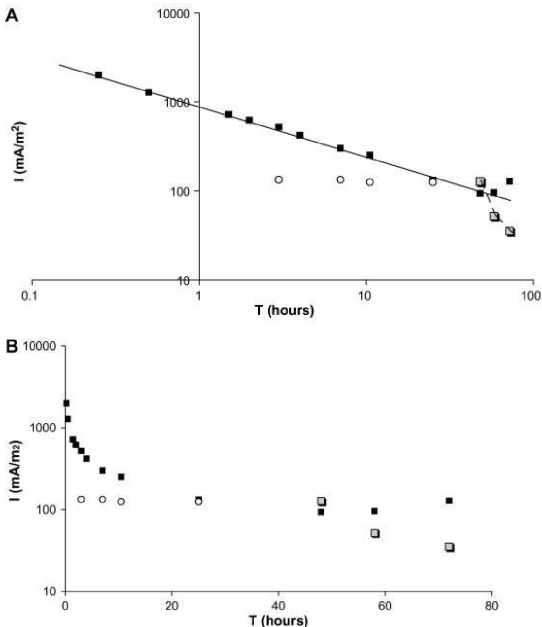
Fig. 4. Evolution of current density ( \text{mA}/\text{m}^2 ) with a new clean electrode ( 2.5 \text{ cm}^2 ) polarized at -100 \text{ mV} vs. \text{Ag}/\text{AgCl} (■); biofilm-covered electrode polarized intermittently (○) and continuously after 48 h (■); interpolation of results: (—) i = 840 \times t^{-0.5} ; (---) i = 180 \times (t - 46)^{-0.5} . (A) In a log–log scale. (B) In a log–regular scale.
