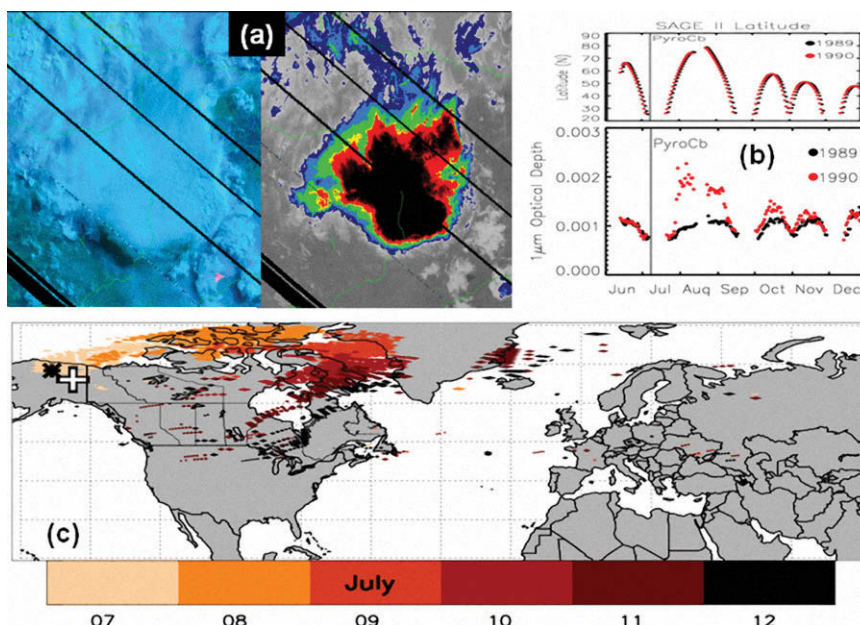
FIG. 3. Composite of AVHRR, AI, and SAGE II AOD for 1990 Circle pyroCb. (a) AVHRR RGB and 11- \mu m BT for morning (1423 UTC) 7 Jul 1990 over northern Alaska. THIR color enhancement for BT < -40°C; black is BT < -57°C. Minimum BT = -65.3°C. (b) SAGE II measurement latitude pattern for (top) 1989 and 1990 and (bottom) daily average LS AOD for Jun through Dec. (c) Map of TOMS AI color coded by date, between 7 and 12 Jul 1990, location of 6 Jul pyroCb (+), and day-after anvil (*).
