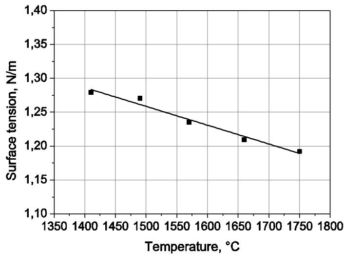
Figure 8. Surface tension of \text{Cu}_{75}\text{Co}_{25} alloy.
