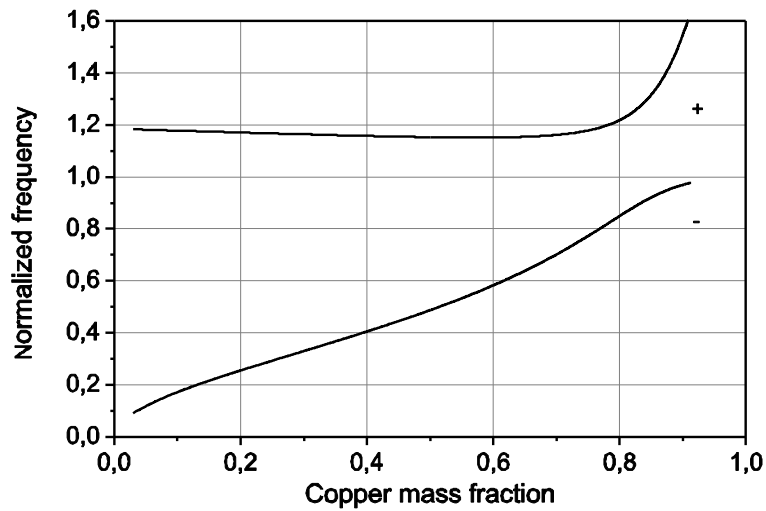
Figure 3. The normalized normal mode frequencies \omega_{\pm}/\omega_0 as a function of the relative mass fraction m_{rel} . For the figure, following parameters were chosen: \sigma_0=1.3 N/m, \sigma_{12}=0.5 N/m, \rho_0=7.75 g/cm 3 , \rho_i=7.86 g/cm 3 .
