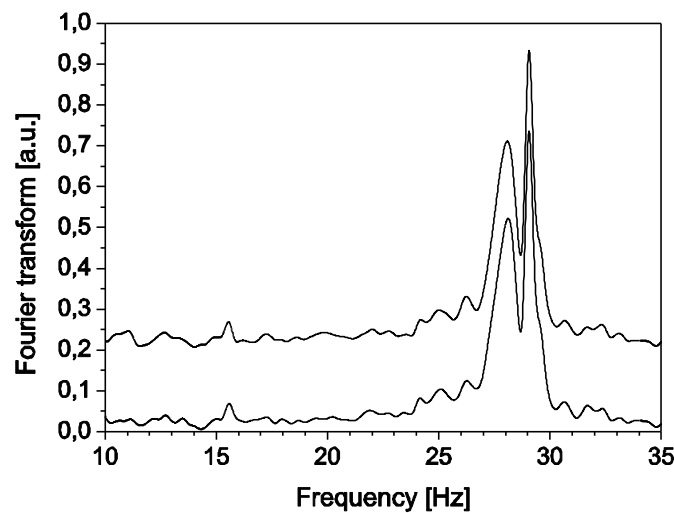
Figure 9. Fourier spectra of the 1 st pulse in the 1 st cycle. FFT of cross section (top) and radius sum (bottom) is shown. Spectra are shifted vertically for clarity.
