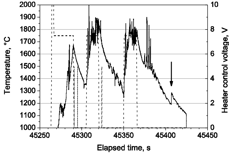
Figure 5. Temperature-time profile of the Cu-Co TEXUS 44 experiment. Dotted lines show the heater activity, not all pulses are shown due to the time resolution of the display. The arrow indicates final solidification.
