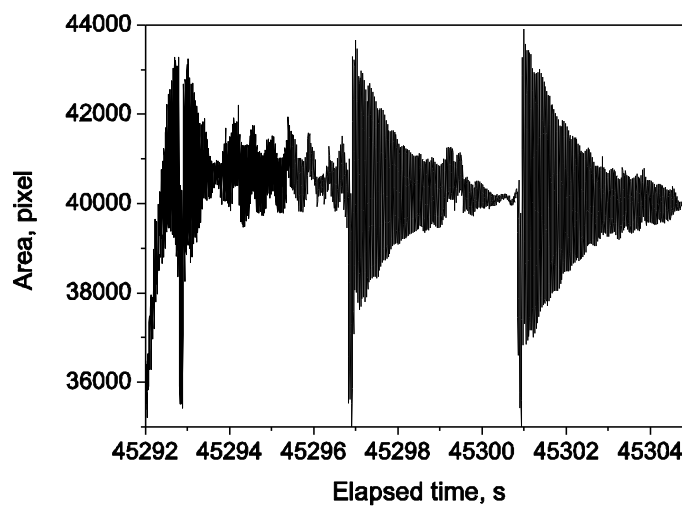
Figure 6. Oscillations of the visible cross section during the first melting cycle.
