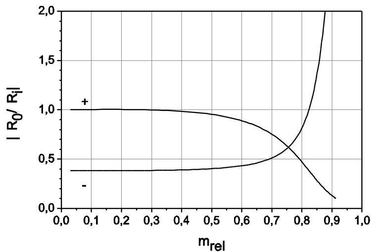
Figure 4. Relative amplitudes of the oscillations of inner and outer surface as a function of mass fraction for both modes.
