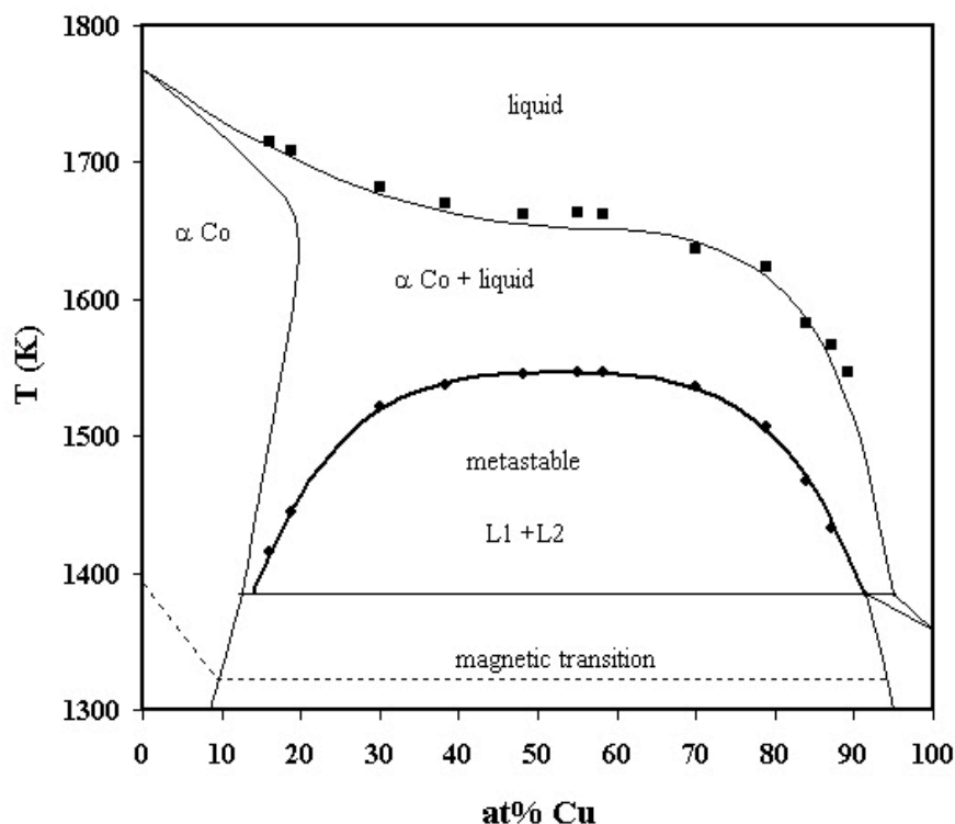
Figure 1. Phase diagram of Cu-Co showing the metastable miscibility gap. Symbols indicate experimentally determined liquidus and binodal temperatures.
