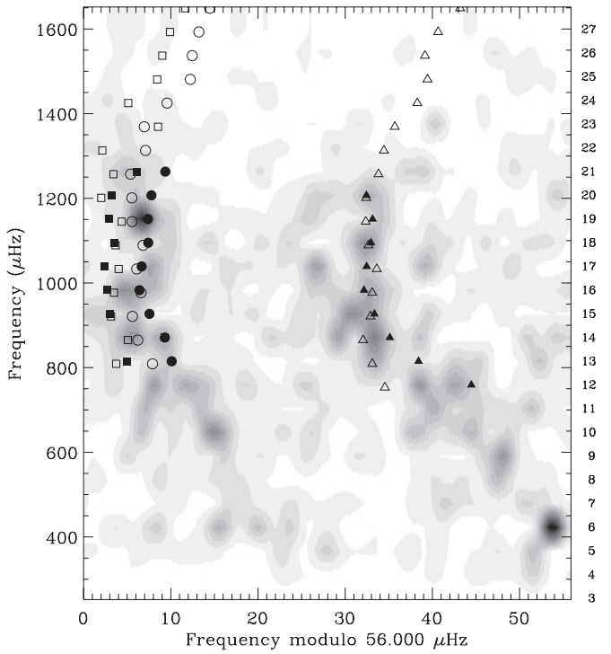
Figure 7. Échelle diagram for Procyon smoothed to 2 \mu\text{Hz} (grayscale) overlaid with scaled frequencies for two stars observed by CoRoT . The filled symbols are oscillation frequencies for HD 49385 reported by Deheuvels et al. (2010), after multiplying by 0.993. Open symbols are oscillation frequencies for HD 49933 from the revised identification by Benomar et al. (2009b, Scenario B) after multiplying by 0.6565. Symbol shapes indicate mode degree: l = 0 (circles), l = 1 (triangles), and l = 2 (squares).
