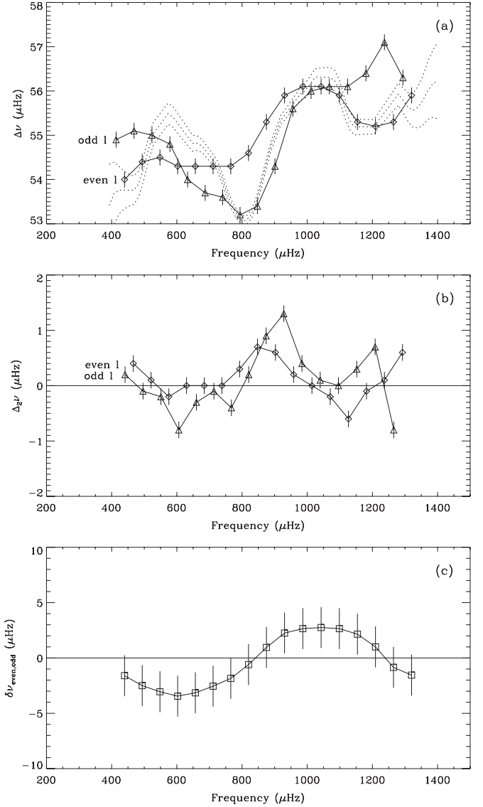
Figure 11. Symbols show the frequency separations in Procyon as a function of frequency, as measured from the ridge centroids: (a) large frequency separation, (b) second differences, and (c) small frequency separation. The dotted lines in panel a show the variation in \Delta\nu (with \pm 1\sigma range) calculated from the autocorrelation of the time series—see the text.
