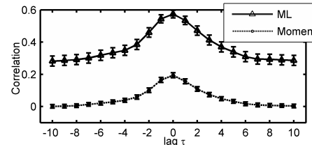
(c) Window Size n = 15 \times 15
