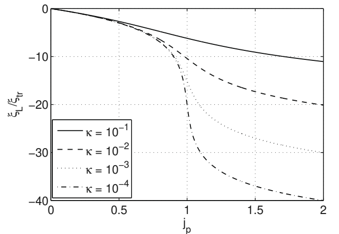
Fig. 8. Threshold-crossing in a microring resonator with an homogeneously broadened atomic transition, as a function of normalized pumping level j_p . Reduced linewidth W = (\xi_L/\xi_{tr}) (with respect to transparency value \xi_{tr} ), expressed in dB, for \kappa = 10^{-1}, 10^{-2}, 10^{-3} and 10^{-4} ; note the high gain of coherence that goes with the passage across threshold.
