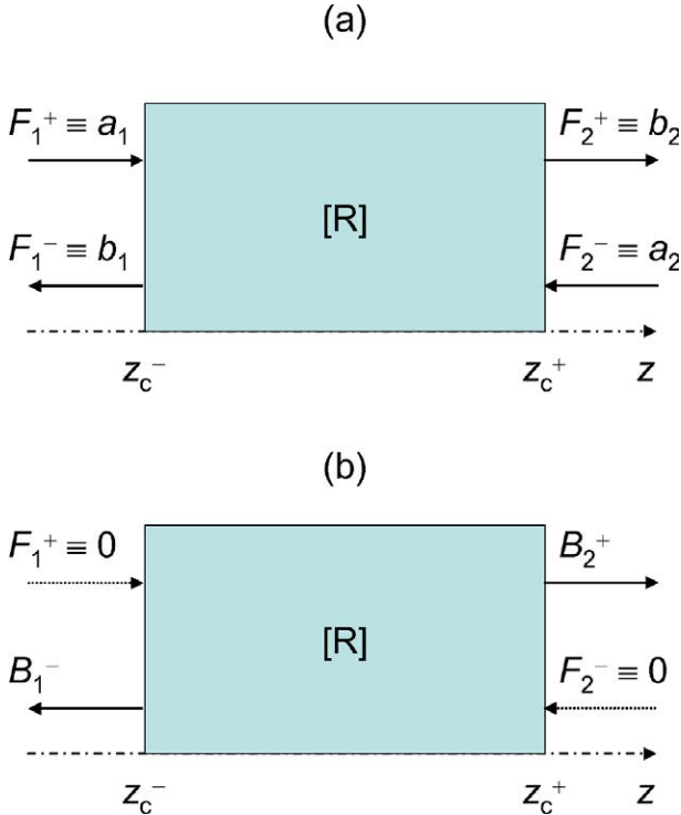
Fig. 4. Notations for extended Transfer Matrix Formalism connecting the co- and contrapropagating waves supported by the straight waveguide: (a) Input/output waves connected through ports (1) and (2) of the system ring + coupler; (b) background output waves ( B_1^-, B_2^+ ) outcoupled from the system when no ingoing wave is present ( F_1^+ = F_2^- = 0 ).
