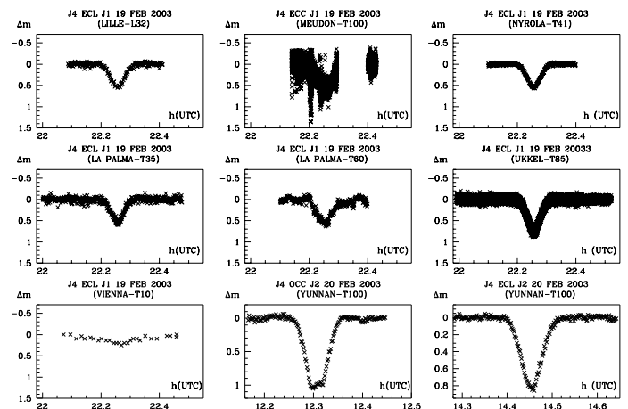
Fig. 18. Light curves for the observations of the mutual events of the Galilean satellites in 2002–2003.
