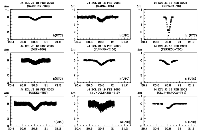
Fig. 16. Light curves for the observations of the mutual events of the Galilean satellites in 2002–2003.
