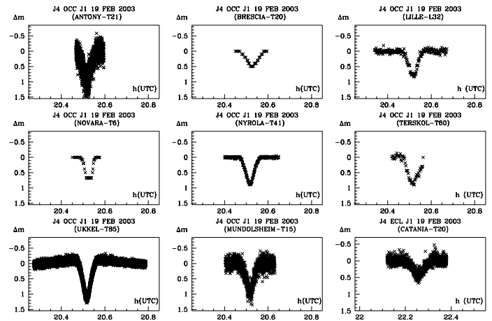
Fig. 17. Light curves for the observations of the mutual events of the Galilean satellites in 2002–2003.
