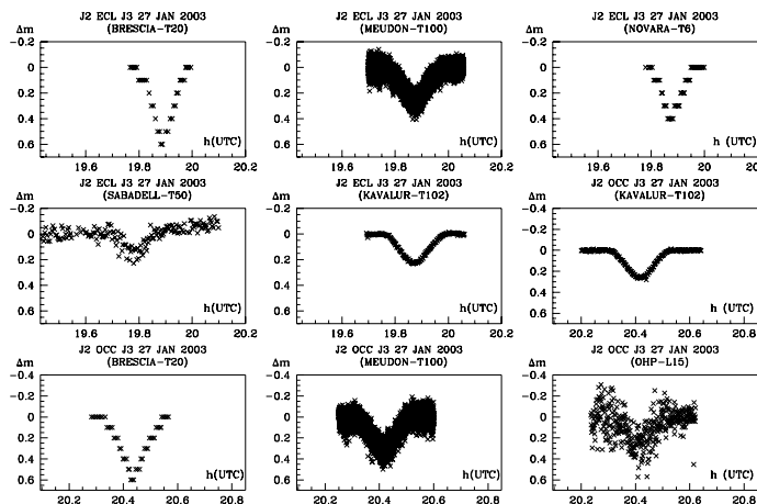
Fig. 11. Light curves for the observations of the mutual events of the Galilean satellites in 2002–2003.
