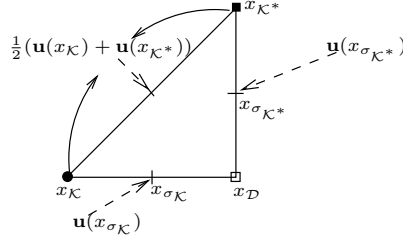
FIG. 6.1. The affine interpolation \mathbb{P}_{\mathbf{c}}^{\mathcal{Q}} on the quarter diamond cell \mathcal{Q} = \mathcal{Q}_{K,K^*} .
