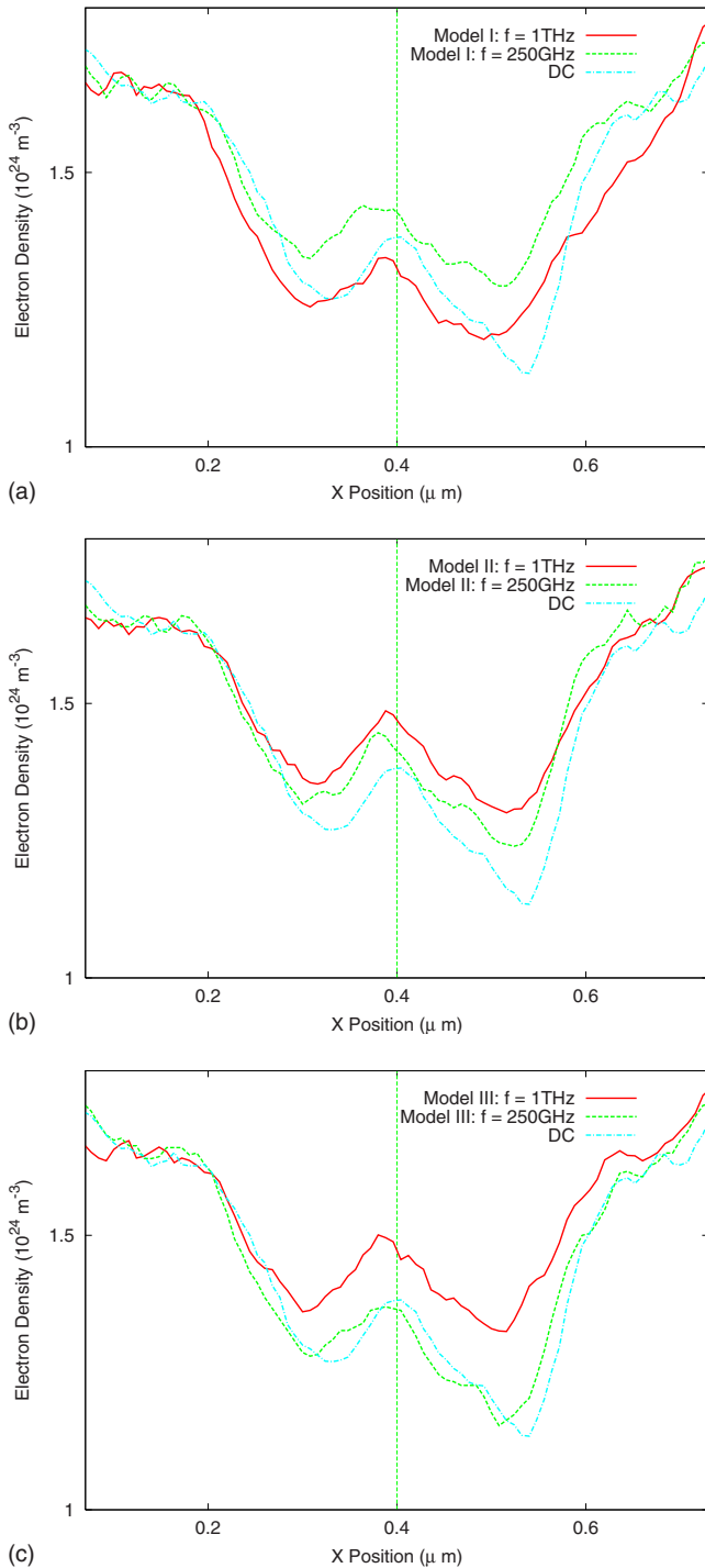
FIG. 9. (Color online) Variations in the mean electron density in the channel at z=0.21 \mu\text{m} , for the dc case, a frequency of 250 GHz, and a frequency of 1 THz, and for surface charge models I (top curve), II (middle curve), and III (bottom curve). For model II, \tau is set to T/5 . The results are for a bias of 0.3 V. The vertical line indicates the center of the device.
