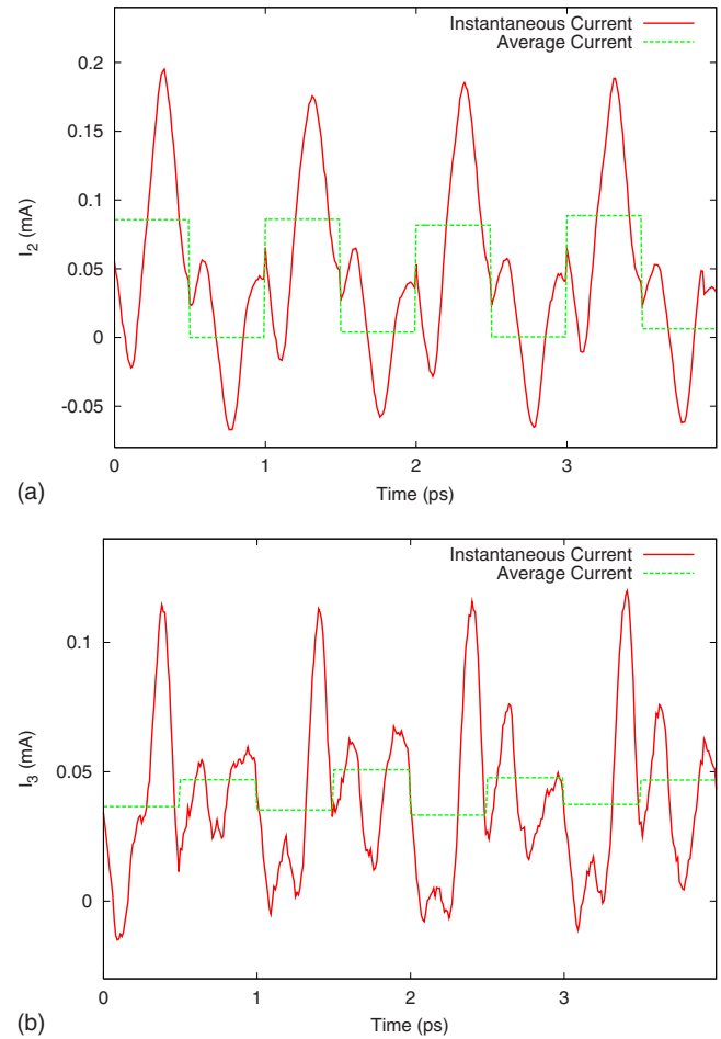
FIG. 12. (Color online) Time variation of the device currents for a 1 THz frequency and surface charge model II ( \tau=T/5 ). The top graph shows the current through the right branch ( I_2 ), and the bottom graph shows the current through the vertical branch ( I_3 ).
