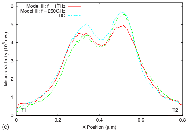
FIG. 7. (Color online) Variations in the mean electron velocity in the x direction in the channel at z=0.21 \mu\text{m} , for the dc case, a frequency of 250 GHz, and a frequency of 1 THz, and for surface charge models I (top curve), II (middle curve), and III (bottom curve). For model II, \tau is set to T/5 . The results are for a bias V of 0.3 V.
