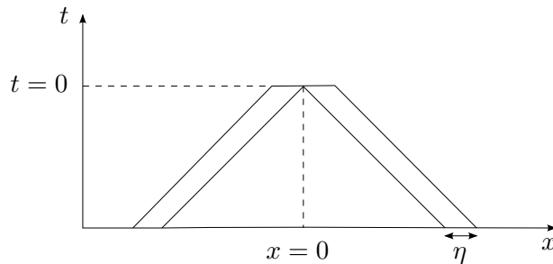
Figure 2: The truncated cone K
