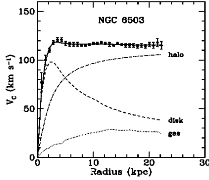
Figure 1: Galaxy rotation curve
